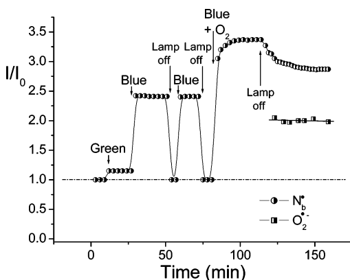
Figure 5. EPR signal intensity of N_b^* and O_2^{\bullet-} in various conditions. I_0 = 1 is the N_b^* intensity in the non-irradiated sample.
